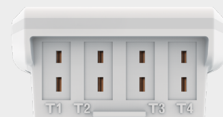
KTT 320: 4 mini-thermocouples connections
